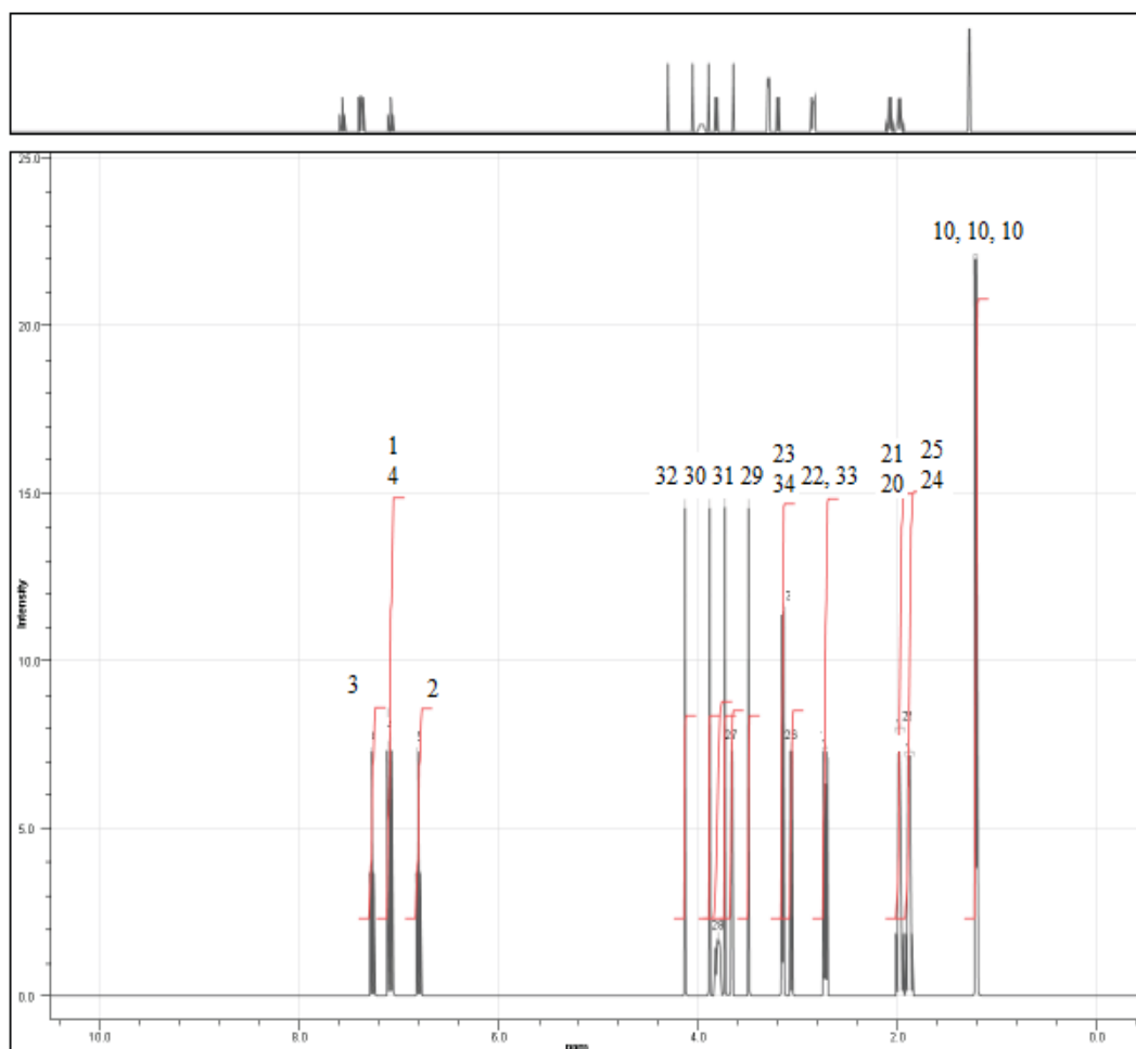
Figure 58: Better resolution of ^1\text{H-NMR} spectrum of (AZ-6) by Marvin Sketch.
